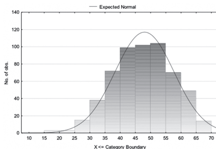
Figure 2: Kolmogorov-Smirnoff test show that distribution of results from both samples do not statistically differ from theoreticly normal distribution ( d1=0,03654 , p1>0,20 ; d2=0,04144 , p1>0,20 ), respectively.
