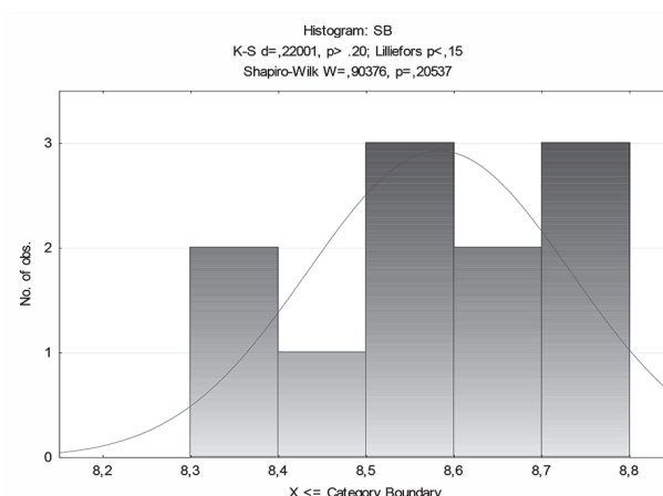
Histogram 2 – SB- normality of distribution
